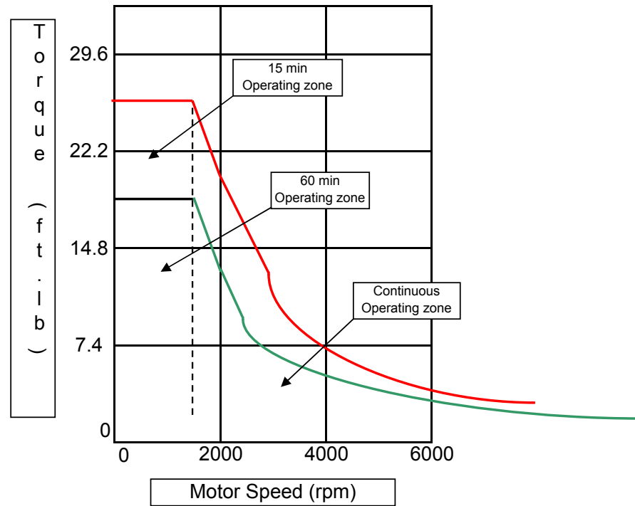
Torque-Motor Speed graph for GT-27 (English)
