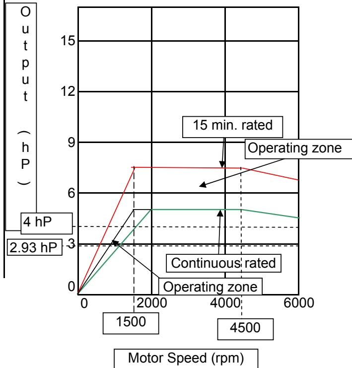
Output -Motor Speed graph for GT-27 (English)
